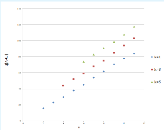
Figure 2: The condition for the second stage of new style diploids to be generated with the higher probability than the first new style diploids. The values of the right hand side of inequality (20) are plotted against the values of \nu in the three cases of \kappa values. In this plotting, the values of P_{r:\nu}/Q_\nu in Figure 1 are used for the values of P_{r:\nu} and P_{r:\kappa} by tentatively assuming Q_\nu and Q_\kappa to be 10^{-2\nu} , and 10^{-2\kappa} , respectively. The inequality (20) holds in the region where the values of (m-\nu)h (longitudinal coordinate) are larger than the values on the plotted curve. For example, more than 16 of (m-\nu)h value is sufficient for the satisfaction of the inequality in the case of \nu=2 and \kappa=1 , but the value of (m-\nu)h amounts to more than 108 in the case of \nu=10 and \kappa=5 .
