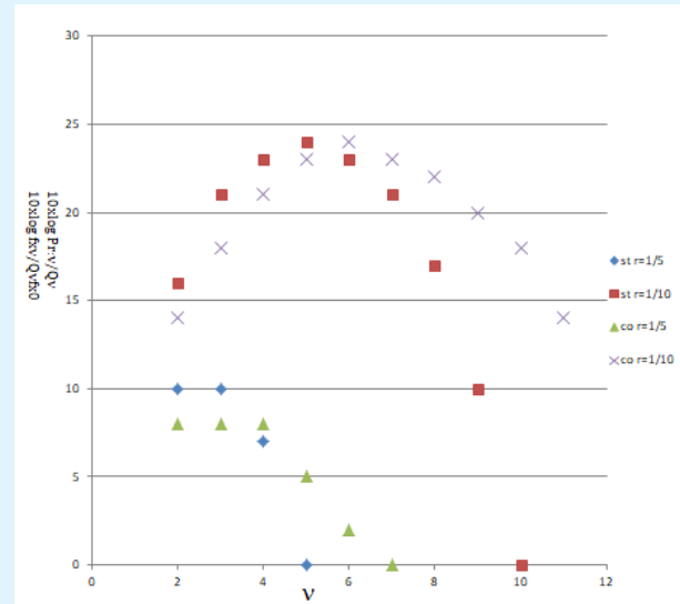
Figure 1: Comparison in accumulating new genes generated from gene duplication between the multiple steps of gene duplication and the exchange homologous chromosomes through conjugation. According to Equation (6), the values of f_{x\nu}/Q_\nu f_{x_0} are plotted against the values of \nu for two cases of r=1/5 and r=1/10 , which are denoted as st\ r=1/5 and st\ r=1/10 , respectively. Although each of these plotted curves takes a maximum value on the way to f_{x\nu}=0 , the values of f_{x\nu} 's are monotonously decreased because the product Q_\nu of mutation rates is more decreased as the number \nu is increased. The values of P_{r:\nu}/Q_\nu calculated on the basis of Equation (8) for the cases of r=1/5 and r=1/10 are also plotted as co\ r=1/5 and co\ r=1/10 , respectively, where P_{r:\nu} of even number \nu is calculated from \nu_1=\nu_2=\nu/2 and that of odd number \nu is calculated from \nu_1=\nu_2+1=(\nu+1)/2 . Although P_{r:\nu}/Q_\nu is slightly smaller than f_{x\nu}/Q_\nu f_{x_0} in the smaller number of \nu , the former becomes certainly larger than the latter in the larger number of \nu for each case of reduction factor r and moreover the number \nu , which gives non-zero probability P_{r:\nu} extends to the region where f_{x\nu} is zero. In the case of r=1/10 , for example, P_{r:\nu} 's are not zero even in the region of \nu from 12 to 19, although they are not shown in the figure for simplicity.
