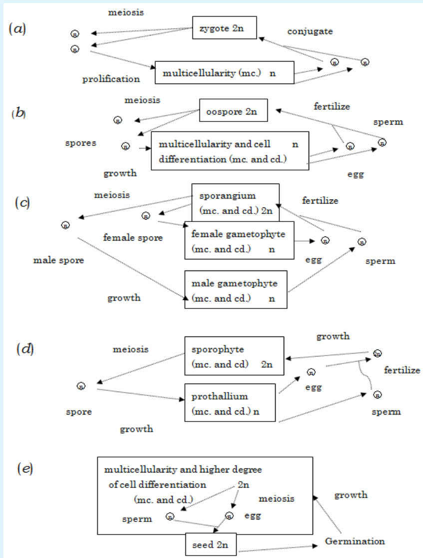
Figure 3: The representative examples of green plants showing the intermediate stages in the innovation from monoploids to diploids along the advancement in cell differentiation. (a) The Conjugatae such as Roya and Spirogyra repeats a cycle of unicellular monoploids, multicellular monoploids, conjugation of two monoploid cells to form a zygote and returning to the unicellular monoploids by meiosis. (b) The Chara of Charophyta develops the multicellularity and cell differentiation in the monoploid state. This adult form produces both eggs and sperms, whose fertilization yields the oospore. By the meiosis, the oospore produces the spores, each of which grows to the adult form. (c) In the Bryophyta , the monoploid generation differentiates into female and male types of gametophytes, and the fertilized egg on the female gametophyte grows to the sporangium which produces both female and male types of spores. (d) The Pterophyta develops the cell differentiation in the diploid generation called the sporophyte to acquire the energy and materials by itself and the monoploid generation called the prothallium is specialized to produce only eggs and sperms. In some species of Pterophyta , the prothallium also differentiates into female and male types. (e) The seed plants, in which the monoploid generation (egg and sperm) is produced in the reproductive organ incorporated into the diploid body, take the energy and materials solely by the cooperative action of differentiated cells in the diploid state and develop the albumen to supply the energy and materials with the seed for its germination.
